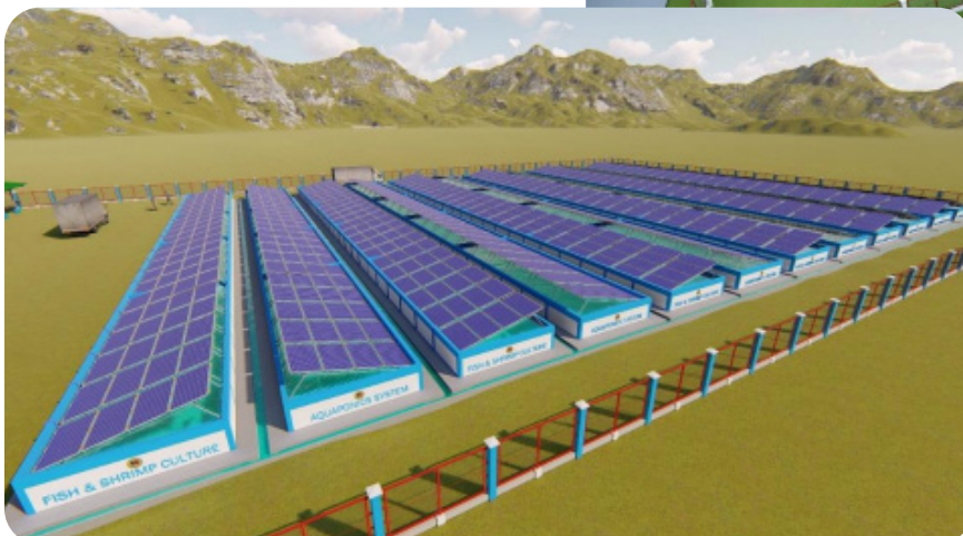
Concrete Fishpond for Fish & Shrimp Culture & Aquaponic System with 518.4 KW Microgrid Solar Power System
